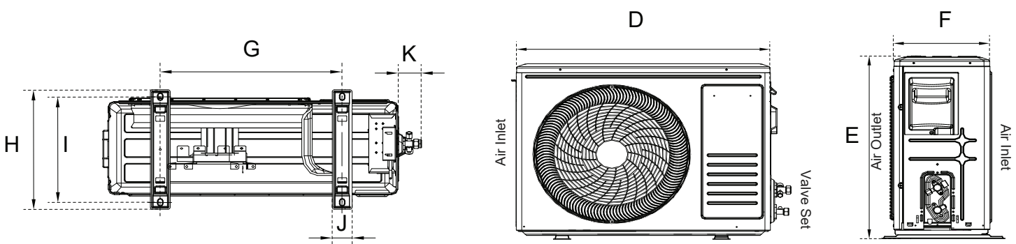
Underside View
