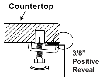
3/8" Positive Reveal
