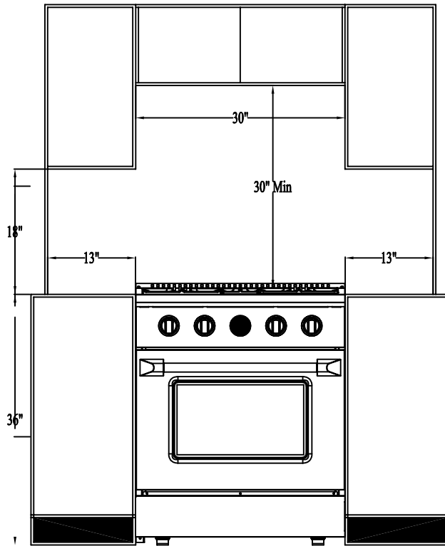
Installation Diagram
