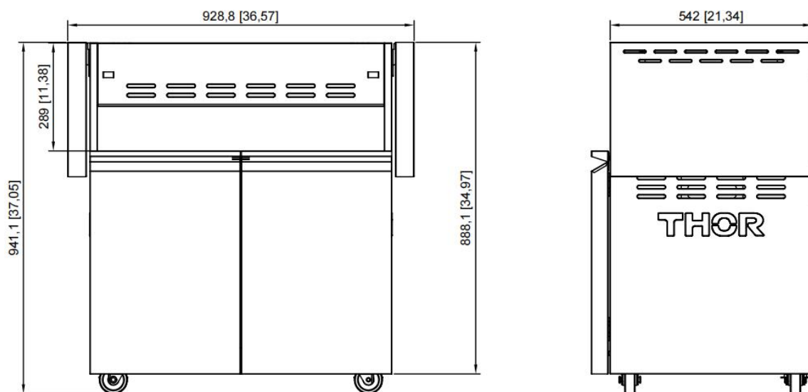
TG32CT – Front & Side View (Side Table Folding)
