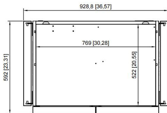
TG32CT – Top View (Side Table Folding)
