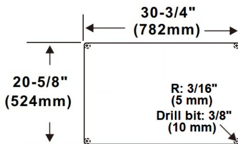
Cutout for Under mount Zero reveal
