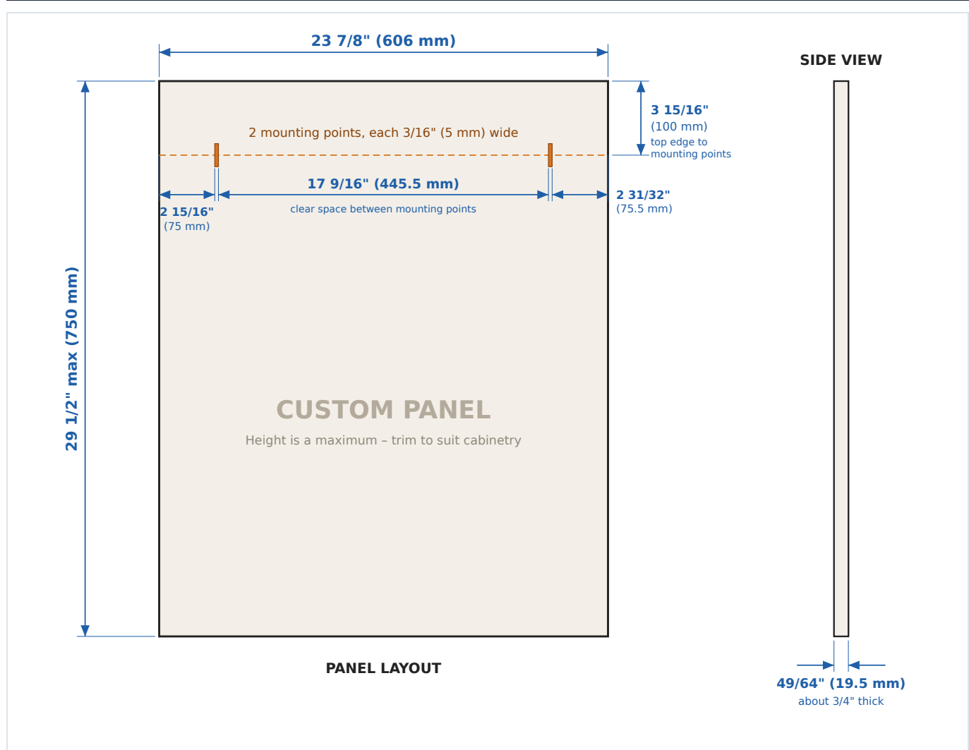
Figure 1. Custom panel layout and side view. Drawn to scale except mounting-point size.
